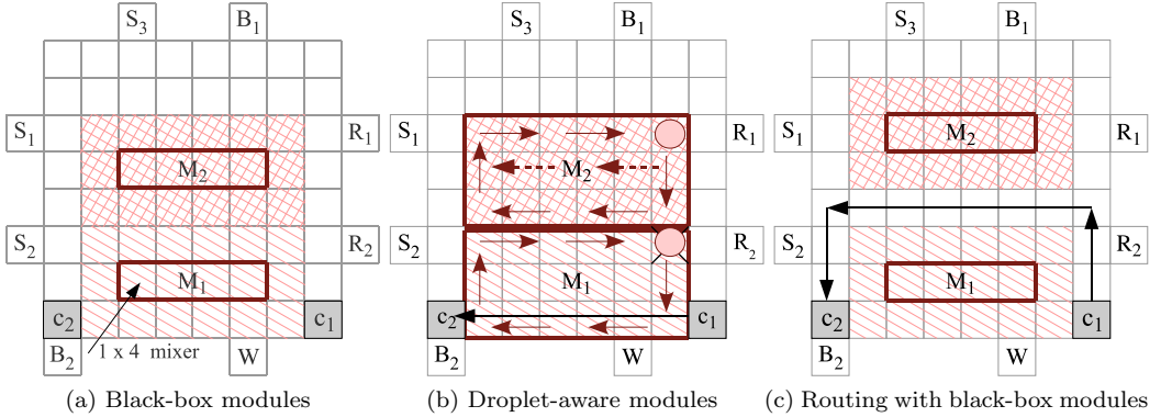
Figure 7.1: Reconfigurable operation execution
