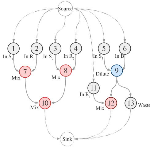
Figure 8.1: Application graph
