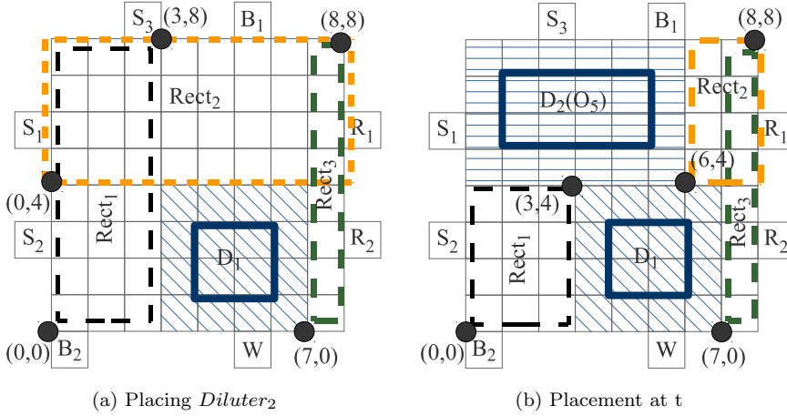
Figure 5.4: Placement example
