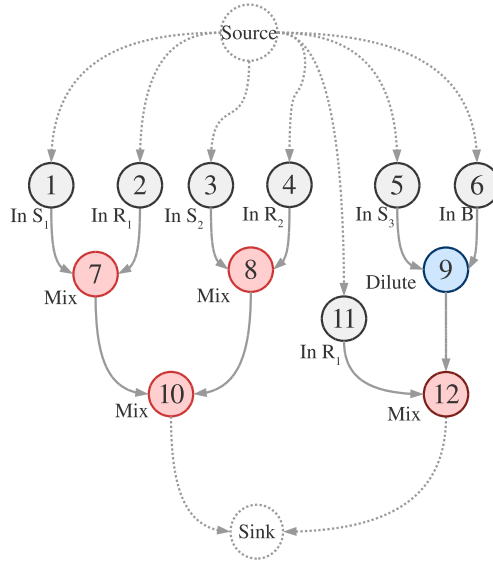
Figure 2.7: Application graph
