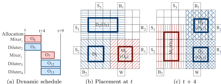
Figure 6.1: Dynamic placement
