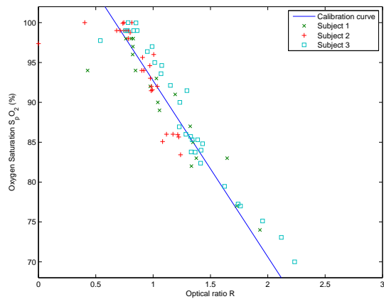
Fig. 7. Calibration curve and estimates obtained using ICAMF. The performance is similar to the DST algorithm, but the algorithm appears to be more robust when considering possible outliers.
