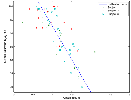
Fig. 5. Calibration curve and estimates obtained using ICAML. Compared to the DST algorithm the estimates deviates more from the calibration curve.
