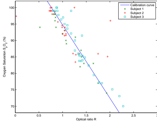
Fig. 3. Calibration curve and estimates obtained using DST. It is seen that the linear model fits most of the estimates, but some estimates could be considered as outliers.
