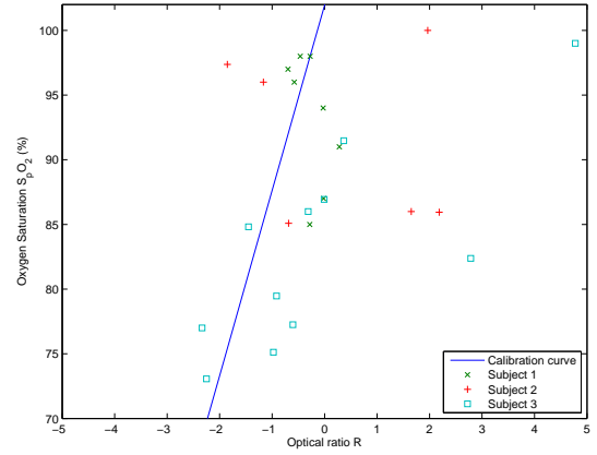
Fig. 4. Calibration curve obtained using FastICA. It is clear that this algorithm fails to estimate R as a most of the estimates are less than zero and the calibration curve has a positive slope. It should be noted that a fewer estimates are seen. This is due to the algorithm not converging for parts of the data.
