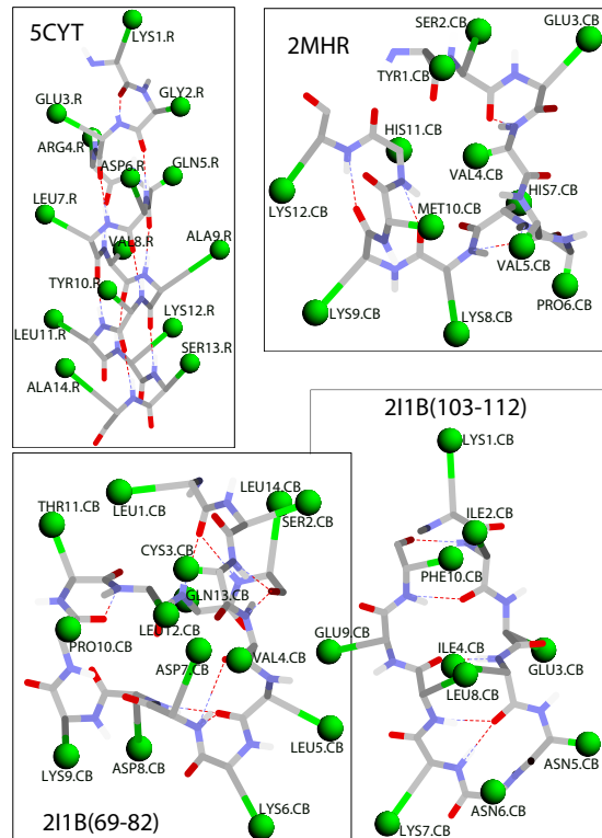
FIG. 3: Color online. Representative decoys from the lowest free energy cluster for four peptides from top left to right (ID, RMSD from native, native structure type): 5CYT 88-101, 1.04Å, \alpha -helix; 2MHR 67-78, 4.74Å, \alpha -helix; 211B 69-82, 4.4Å, \beta -turn and 211B 103-112, 1.63Å, \beta -turn .
