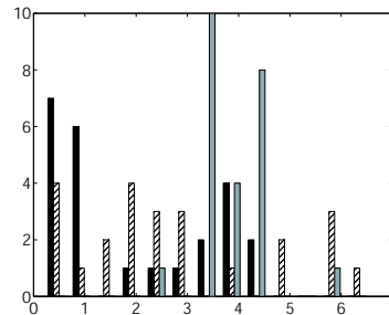
FIG. 2: The RMSD histogram for the minimum free energy conformations for the 24 peptides after training (black), the results for an all-atom potential [20] (hatched) and prior to training (gray).
