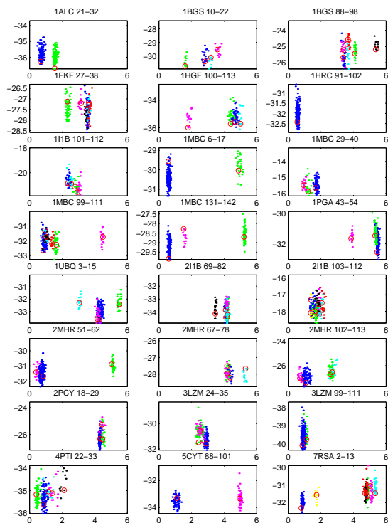
FIG. 1: Color online. Decoy plots – energy versus RMSD ( \text{\AA} ). Cluster RMSD cut-off is 0.5 \text{ \AA} . Cluster centers are marked with a circle. Blue codes for the largest cluster.
