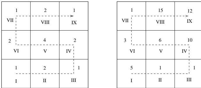
Figure 7.2: Arrival intensity weights for Scenarios A - Narrow/A - Wide and B - Narrow/B - Wide respectively.
