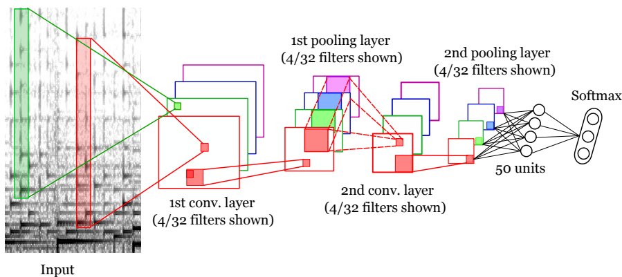
Fig. 1. Illustration of the CDNN architecture we use for our experiments. The CDNN first applies narrow vertical filters to the input sonogram (left) to capture the harmonic structure (we show only 4 of 32). The convolutional layer is cascaded with a max-pooling layer which downsamples the output. This is followed by a 2nd pair of convolutional and max-pooling layers. Finally, the output of the final max-pooling layer is fully connected to a final hidden layer of 50 units, followed by a softmax output unit (giving posterior probabilities of over the set of class labels). The input spectrogram contains 100 time slices sampled every 23ms, which means that the final layer of the CDNN summarises information over a total duration of 2.3 seconds.
