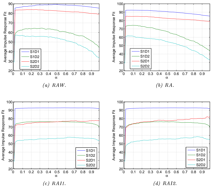
Figure 4.9: OE models - Average impulse response fits achieved by the statistical tests on the residuals as function of the adopted significance level \alpha . The average is calculated from the identification of 200 systems in each data set.
