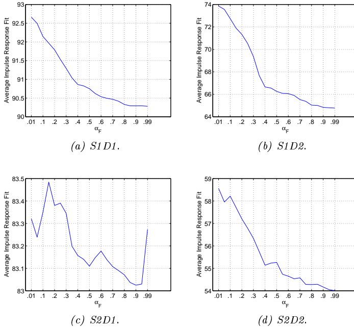
Figure 4.26: OE models - Average impulse response fits achieved for different values of the significance level \alpha_F used in the F-test when it is applied after cross-validation in order to evaluate model structures with increasing complexity. The average is calculated from the identification of 200 systems in each data set.
