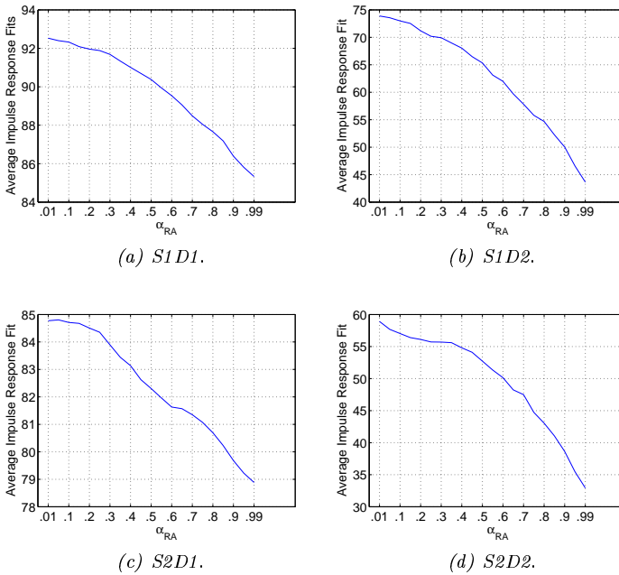
Figure 4.22: OE models - Average impulse response fits achieved for different values of the significance level \alpha_{RA} used in both the tests on residuals (RA) when they are combined with cross-validation for model order selection in the identification of 200 systems in each data set.
