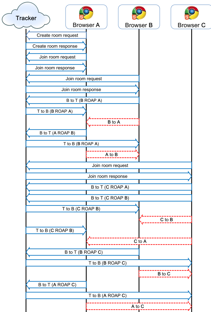
Figure 5.2: Message Sequence for Video Conferencing (Channel Mixing)
