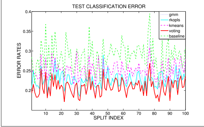
Figure 4. Voting results. It gives the voting performance among GMM, rKOPLS and K-means. The light dash line shows the baseline of random guessing for each data split.
