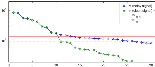
Figure 3. The singular values of the Hankel matrices \bar{H} (clean signal) and H (noisy signal). The solid horizontal line is the “safeguarded” threshold \sqrt{2} m^{1/2} \eta ; the numerical rank with respect to this threshold is k = 13 .
