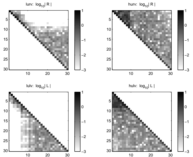
Figure 4. The large and small singular values are reflected in the size of the elements in the matrices R and L from the URV and ULV decompositions. The triangular matrices from the lurv and luLv algorithms (left plots) are closer to block diagonal form than those from the hurv and hulv algorithms (right plots).
