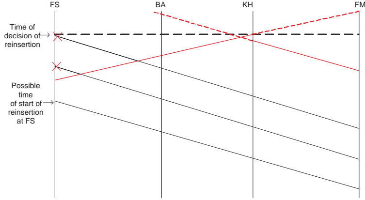
Fig. 5. Illustration of the reinsertion start time at the FS depot. From the decision of reinsertion until the reinsertion can begin at the FS depot, there are two scheduled trains that can not be reinserted as the driver-carrying train has not yet reached the depot
