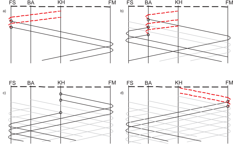
Fig. 6. Illustration of a reinsertion. In a) trains are inserted from depot FS, in b) from depot BA, in c) from KH and in d) from FM.
