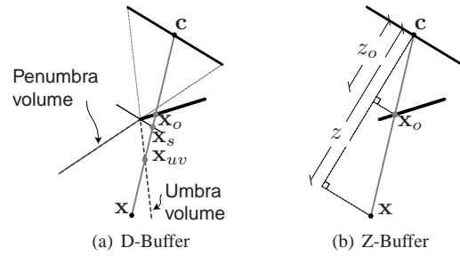
Fig. 5. Difference between shadow map and D-buffer. In the shadow map, only z_o is stored, whereas the D-Buffer stores the distances |\mathbf{c}\mathbf{x}_o| , |\mathbf{c}\mathbf{x}_{uv}| ( |\mathbf{c}\mathbf{x}_{pv}| ) and |\mathbf{c}\mathbf{x}_s|
