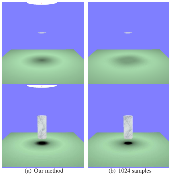
Fig. 7. Scene as in Figure 1 where the umbra region is determined correctly. 7(a) is rendered with our method, and 7(b) is ray traced using 1024 samples of the light source
