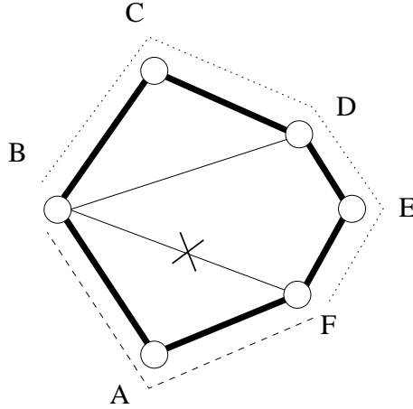
Figure 2: Straddling link protection
