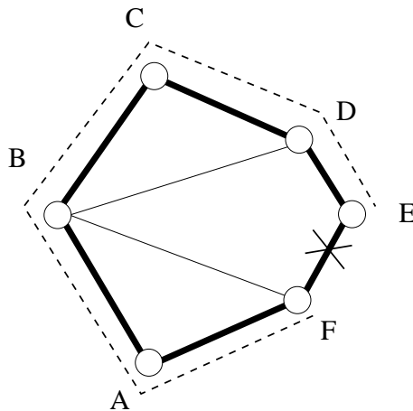
Figure 1: On-cycle link protection
