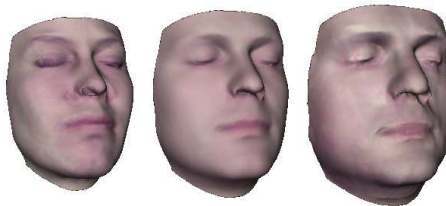
Figure 1: Mode 1 (10%). Left to right represents -3, 0 and +3 standard deviations.
