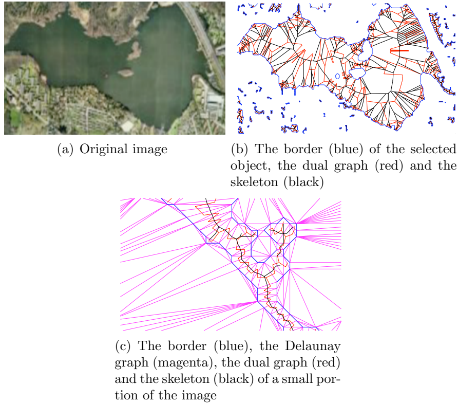
FIGURE 8. The medial axis of a remote sensing image of a lake of Lyngby (Denmark)
