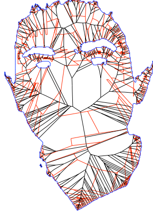
(b) The boundaries of the selected objects, the dual graph and the medial axis
