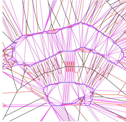
(c) The boundaries, the Delaunay graph, the dual graph and the medial axis of a small portion of the image
