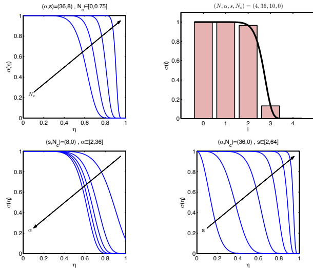
Exponential cut-off filter damping profiles for different parameters.
