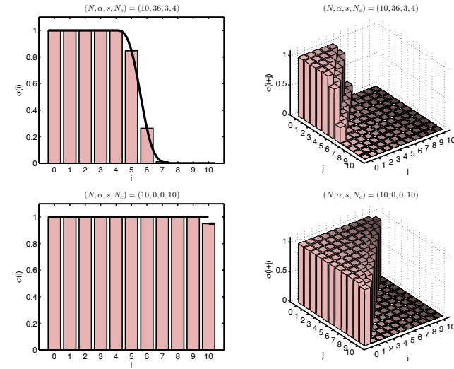
Examples of exponential cut-off filter damping profiles.
