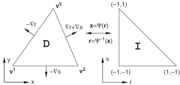
Fig. 6.1. Notation for the mapping between two simplices.
